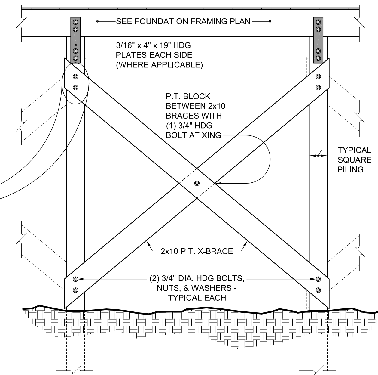
OH15 TYPICAL X-BRACING DETAIL NOT TO SCALE Details Developed By APPIAN Consulting Engineers DATE: 4-6-17
